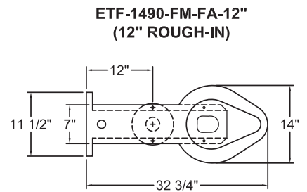
PLAN VIEW
